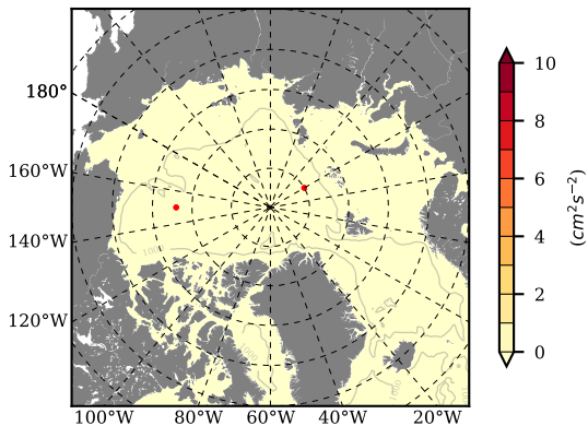
NEMO420WND mean EKE @ 0 m over 1991
