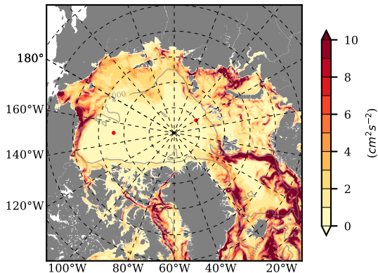
BCTGE27NTMX mean EKE @ 0 m over 1959
