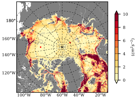
BCTGE27NTMX mean EKE @ 0 m over 1961
