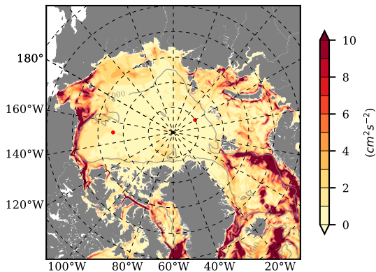
BCTGE27NTMX mean EKE @ 0 m over 1962
