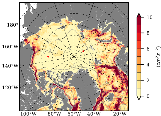
BCTGE27NTMX mean EKE @ 0 m over 1963
