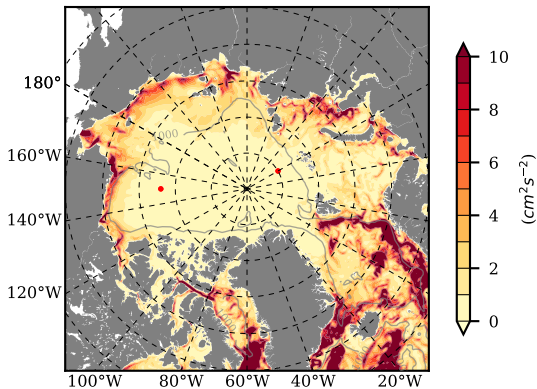
BCTGE27NTMX mean EKE @ 0 m over 1965
