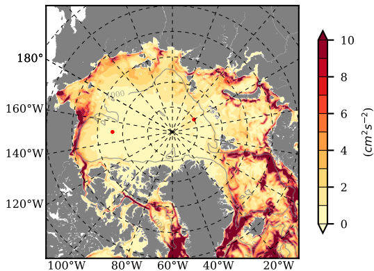
BCTGE27NTMX mean EKE @ 0 m over 1966
