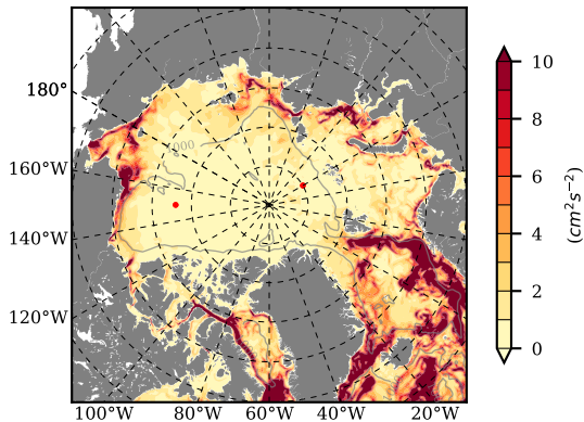
BCTGE27NTMX mean EKE @ 0 m over 1967
