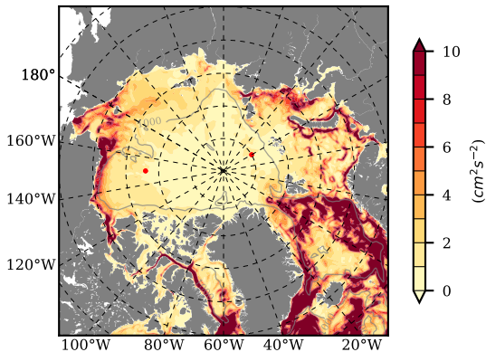
BCTGE27NTMX mean EKE @ 0 m over 1969
