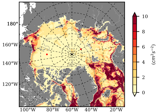
BCTGE27NTMX mean EKE @ 0 m over 1972
