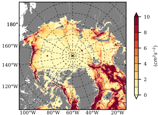
BCTGE27NTMX mean EKE @ 0 m over 1973
