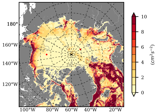
BCTGE27NTMX mean EKE @ 0 m over 1974
