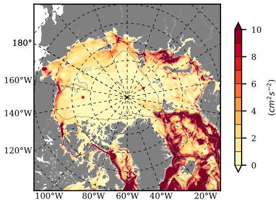
BCTGE27NTMX mean EKE @ 0 m over 1975
