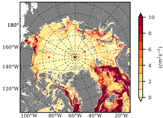
BCTGE27NTMX mean EKE @ 0 m over 1976
