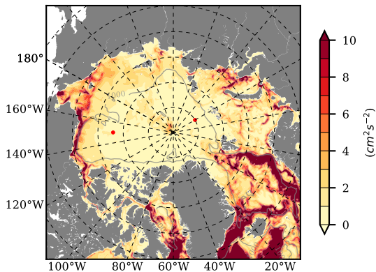
BCTGE27NTMX mean EKE @ 0 m over 1977
