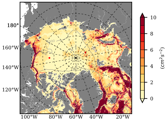
BCTGE27NTMX mean EKE @ 0 m over 1979
