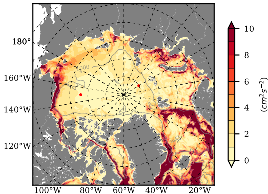
BCTGE27NTMX mean EKE @ 0 m over 1980
