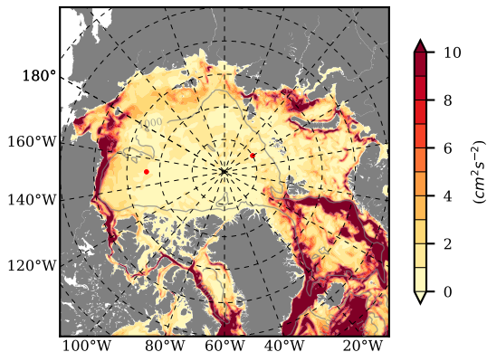
BCTGE27NTMX mean EKE @ 0 m over 1981
