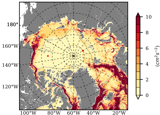
BCTGE27NTMX mean EKE @ 0 m over 1982
