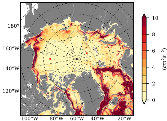
BCTGE27NTMX mean EKE @ 0 m over 1983
