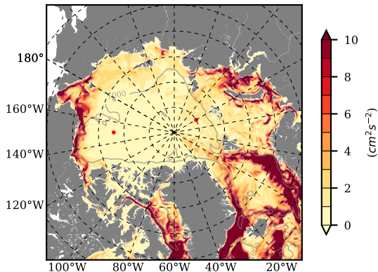
BCTGE27NTMX mean EKE @ 0 m over 1986
