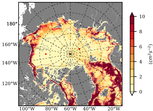
BCTGE27NTMX mean EKE @ 0 m over 1988
