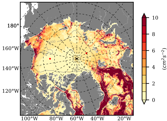
BCTGE27NTMX mean EKE @ 0 m over 1990
