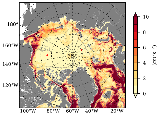
BCTGE27NTMX mean EKE @ 0 m over 1992
