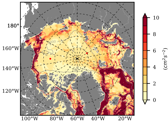
BCTGE27NTMX mean EKE @ 0 m over 1993
