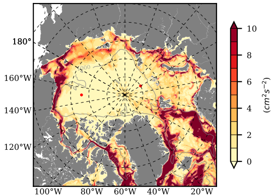
BCTGE27NTMX mean EKE @ 0 m over 1994
