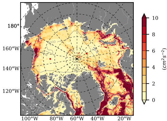
BCTGE27NTMX mean EKE @ 0 m over 1996
