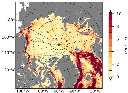
BCTGE27NTMX mean EKE @ 0 m over 1998
