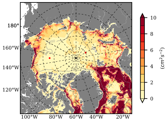
BCTGE27NTMX mean EKE @ 0 m over 1999
