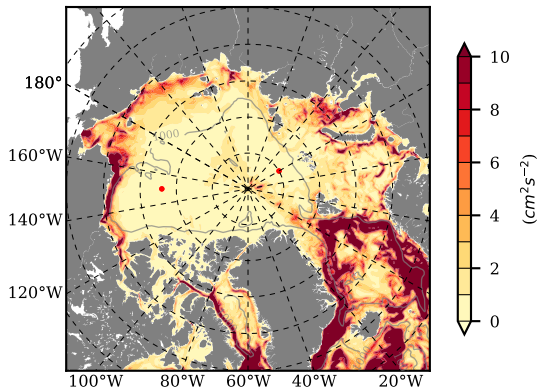
BCTGE27NTMX mean EKE @ 0 m over 2000
