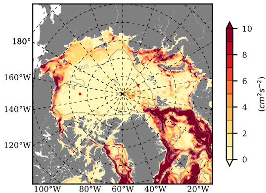
BCTGE27NTMX mean EKE @ 0 m over 2001
