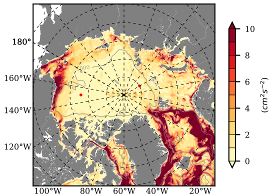
BCTGE27NTMX mean EKE @ 0 m over 2002
