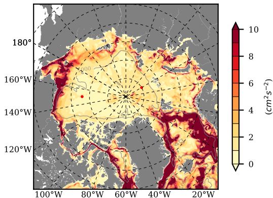
BCTGE27NTMX mean EKE @ 0 m over 2003
