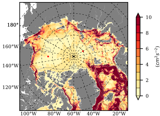
BCTGE27NTMX mean EKE @ 0 m over 2005
