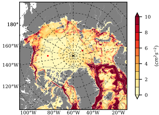
BCTGE27NTMX mean EKE @ 0 m over 2006
