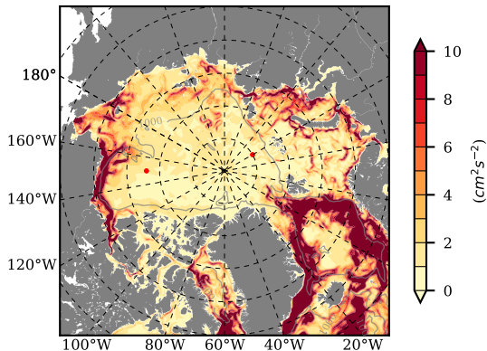
BCTGE27NTMX mean EKE @ 0 m over 2007
