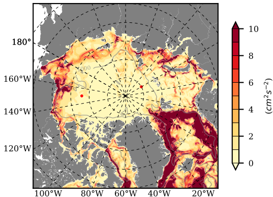
BCTGE27NTMX mean EKE @ 0 m over 2008
