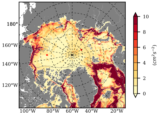
BCTGE27NTMX mean EKE @ 0 m over 2009
