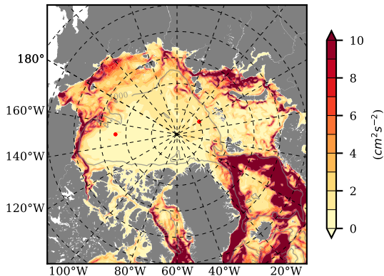
BCTGE27NTMX mean EKE @ 0 m over 2011
