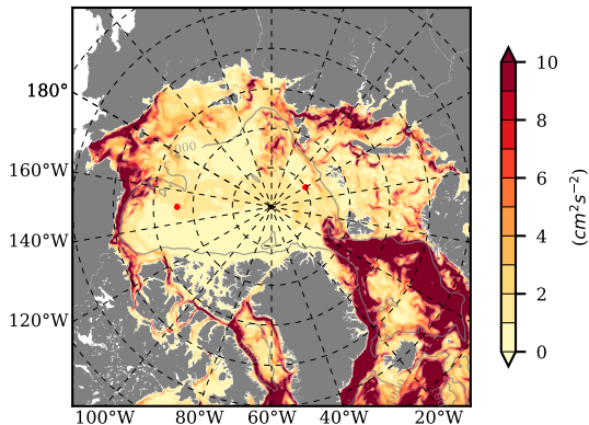
BCTGE27NTMX mean EKE @ 0 m over 2012
