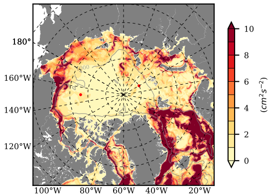
BCTGE27NTMX mean EKE @ 0 m over 2013
