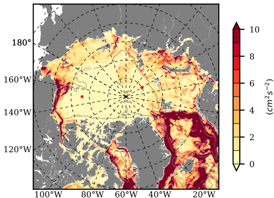
BCTGE27NTMX mean EKE @ 0 m over 2014
