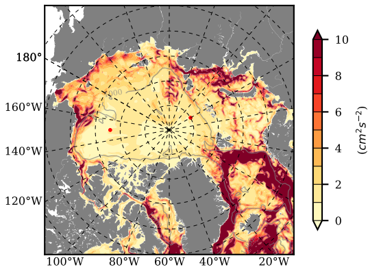
BCTGE27NTMX mean EKE @ 0 m over 2015
