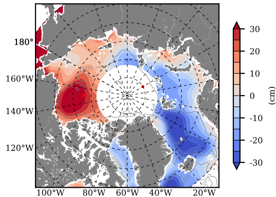
Mean SSH from Armitage et al. 2017 2003-2014
