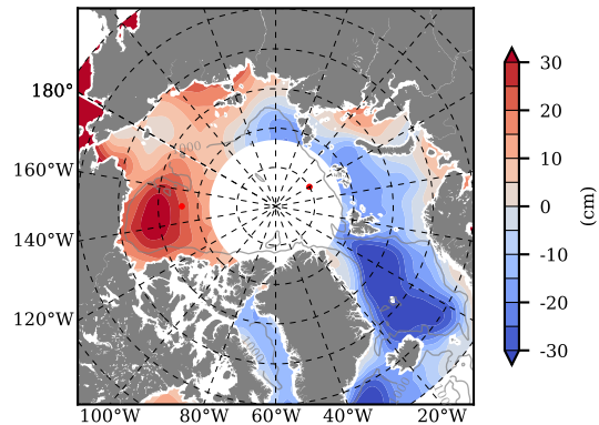
Mean SSH from Armitage et al. 2017 2006
