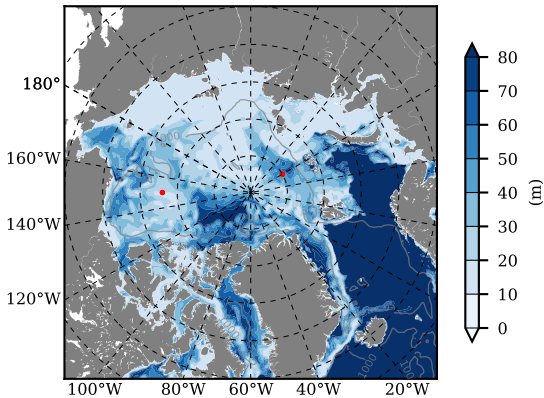
BCTGE27NTMX mean MLD01 over 1999 m03
