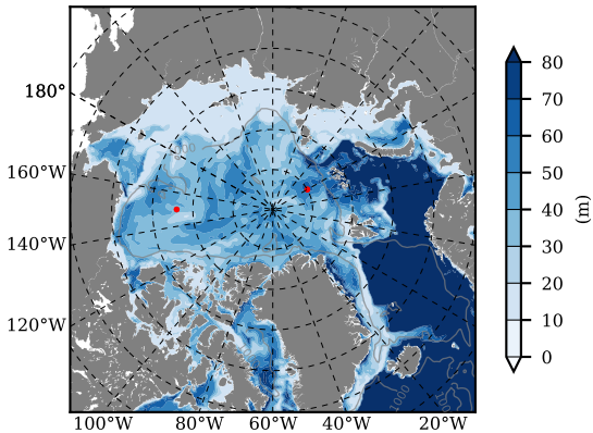
BCTGE27NTMX mean MLD01 over 2011 m03
