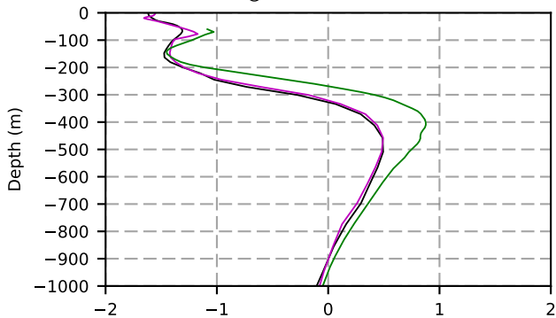
1960 mean temperature @ moor Arctic B box
