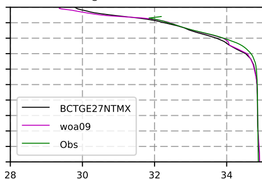
1960 mean Salinity @ moor Arctic B box
