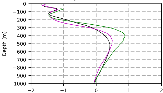
1970 mean temperature @ moor Arctic B box
