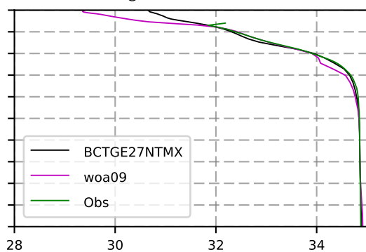
1970 mean Salinity @ moor Arctic B box
