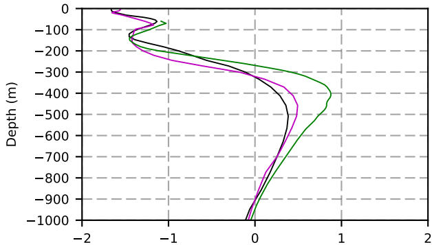
1971 mean temperature @ moor Arctic B box
